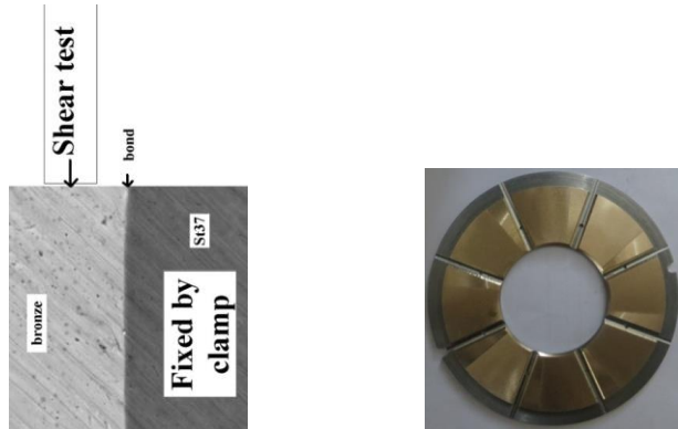
(a) Shear test procedure (b) Final product of axial bearing
